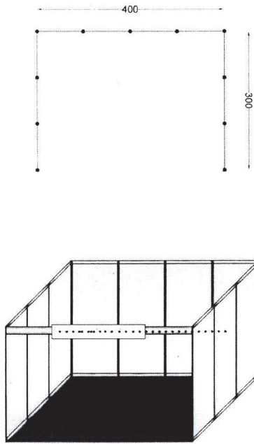
TYPE „A“ BASIC ARRANGEMENT
